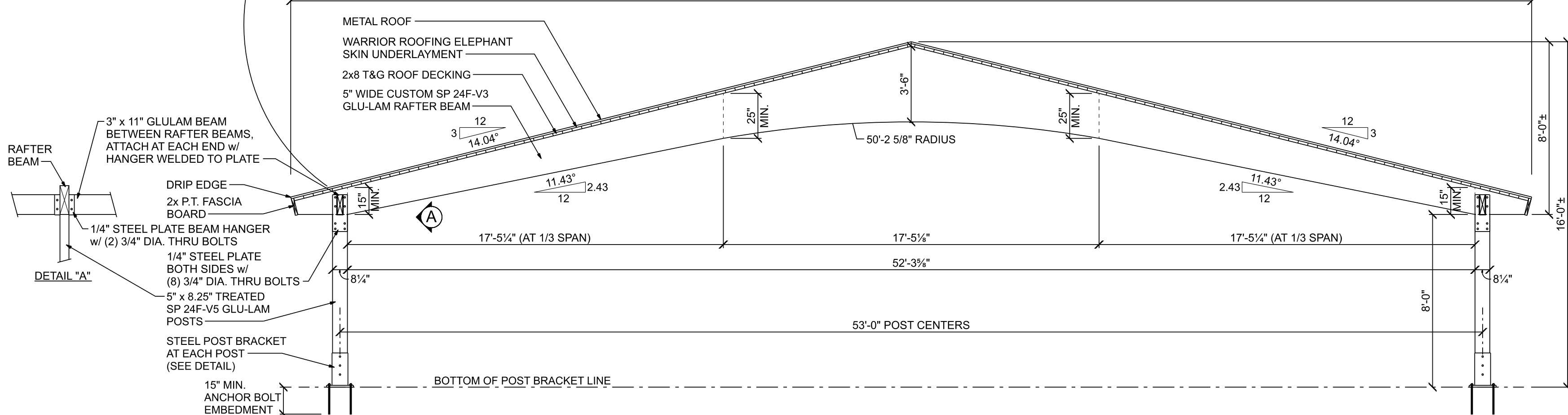
CROSS SECTION
