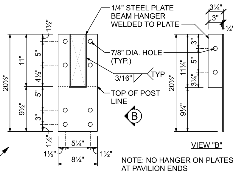
1/4" STEEL PLATE / HANGER DETAIL SCALE: 1" = 1'-0"
