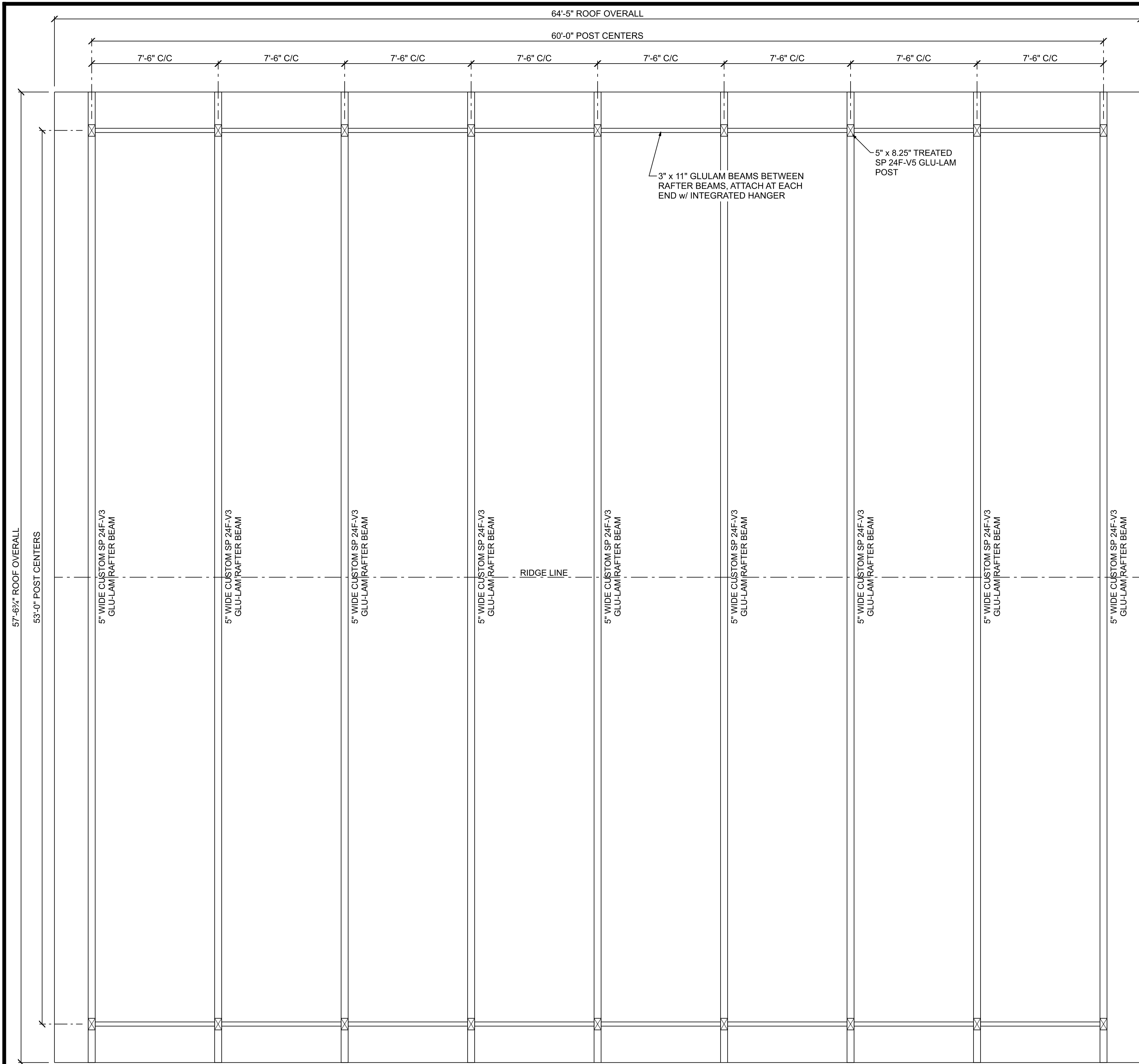
PLAN VIEW
