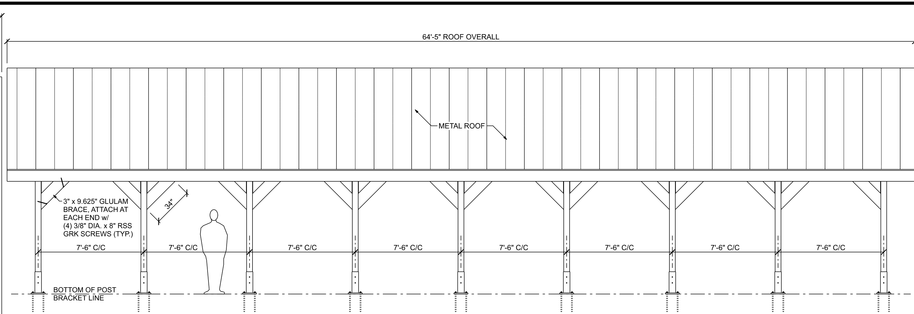
SIDE ELEVATION
