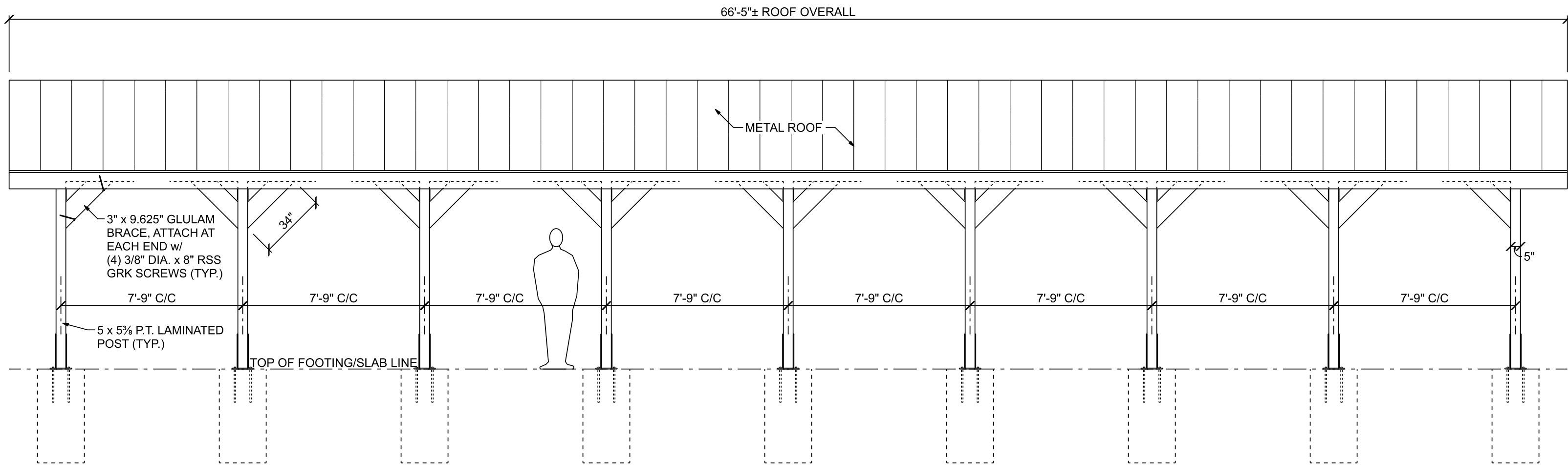
SIDE ELEVATION
