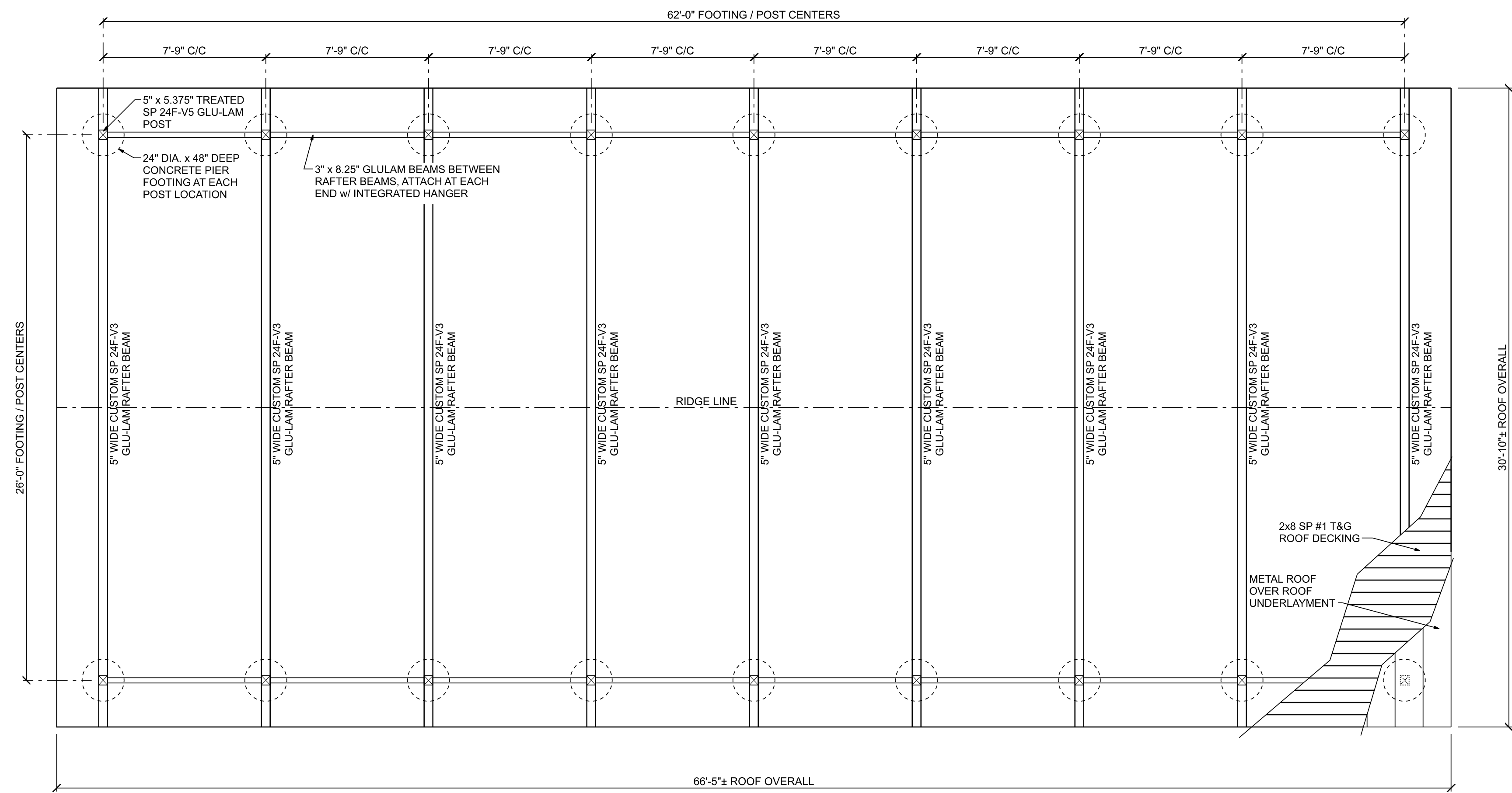
PLAN VIEW
